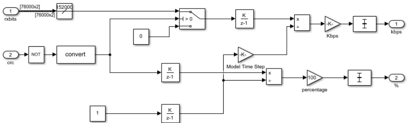
Throughput calculation in percentage and kbps: a) When a subframe has an error, the entire subframe is discarded. b) When two or more codewords are transmitted per subframe, the average throughput is calculated.
